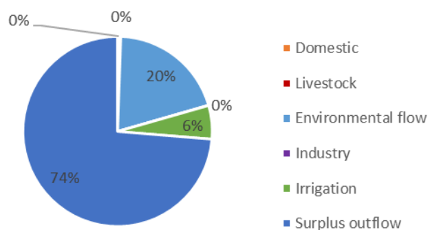
Figure 14: Annual water allocation per water use sector, baseline scenario (source: WEAP model, WRMD, 2018)
