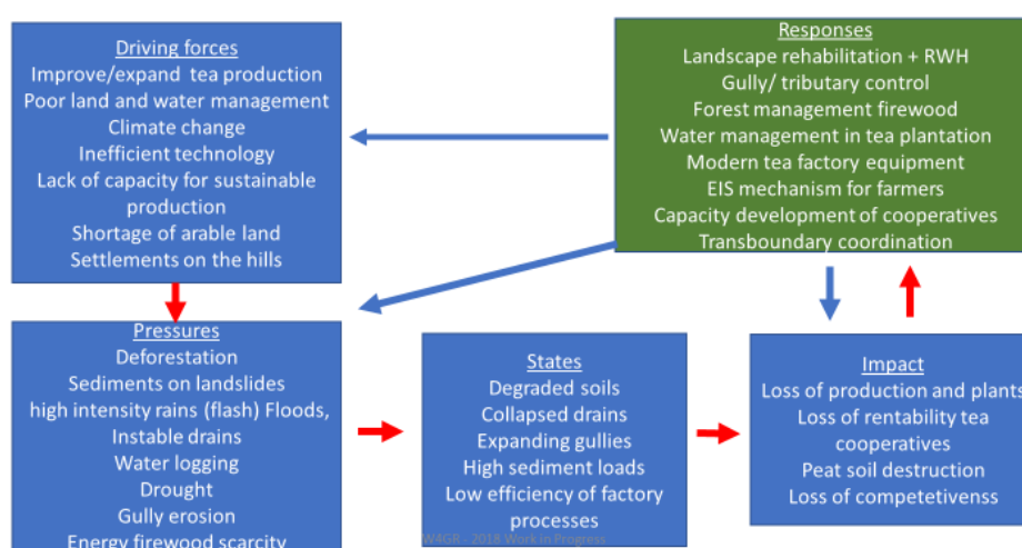
Figure 30: Focused DPSIR analysis for IWRM package 'Support improvements in sustainable water and catchment management (floods and sediments mitigation) through developing the tea and forestry value chains in Mulindi'
