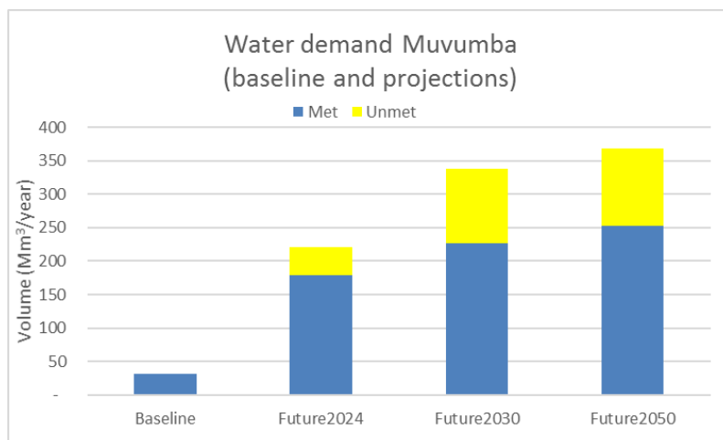
Figure 18: Baseline / projections of met and unmet water demand (water shortage) up to 2050, BaU (W4GR, 2017)
