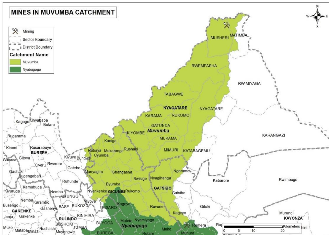
Figure 58: Water Users Survey – Mines in Muvumba catchment
