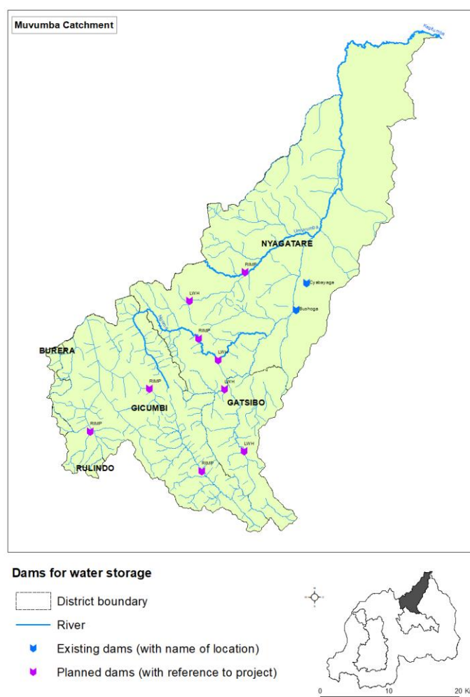
Figure 24: Map of existing and planned dams in the catchment
