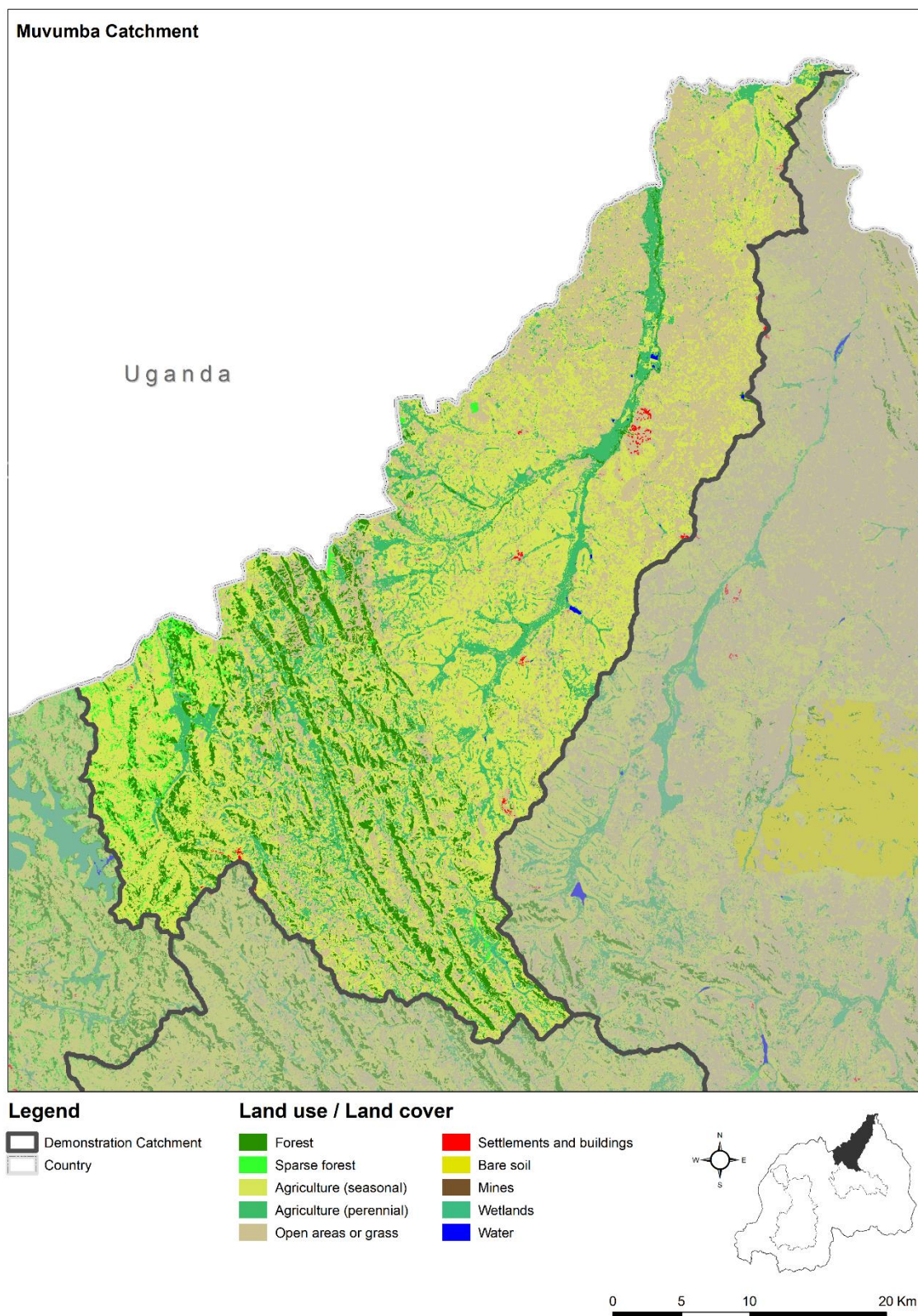
Figure 43: Land Use / Land Cover map (LULC) (W4GR 2018)
