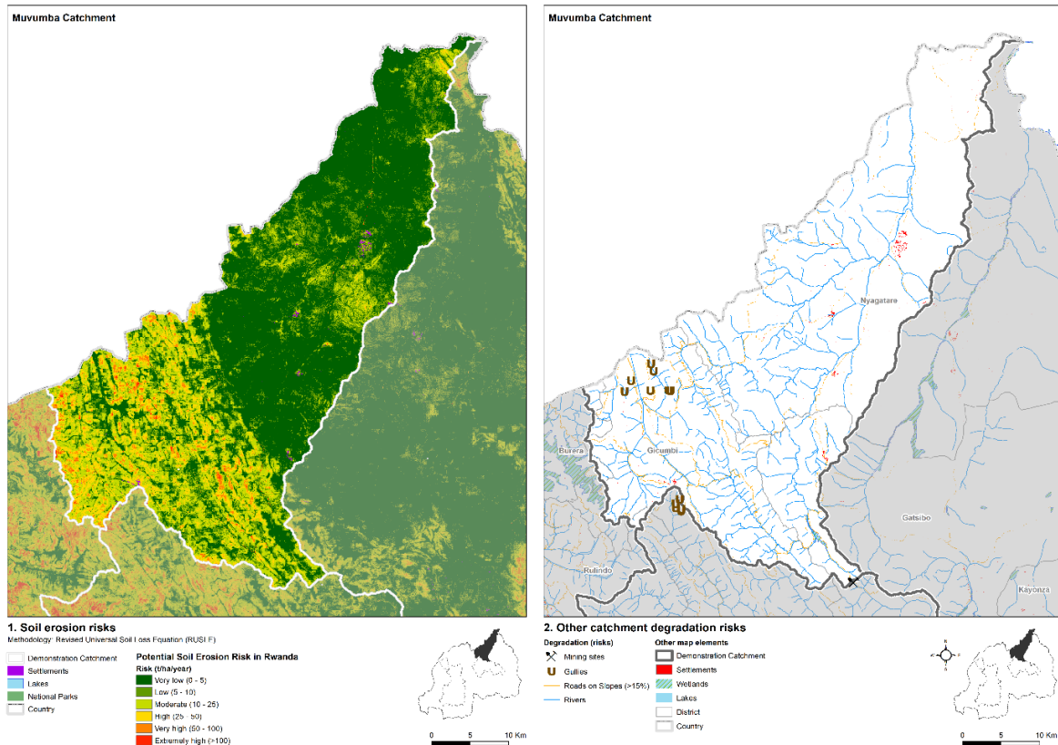
Figure 4: Muvumba Catchment degradation (risk) areas maps (1. Soil erosion risks and 2. Other catchment degradation risks) (W4GR, 2018)
