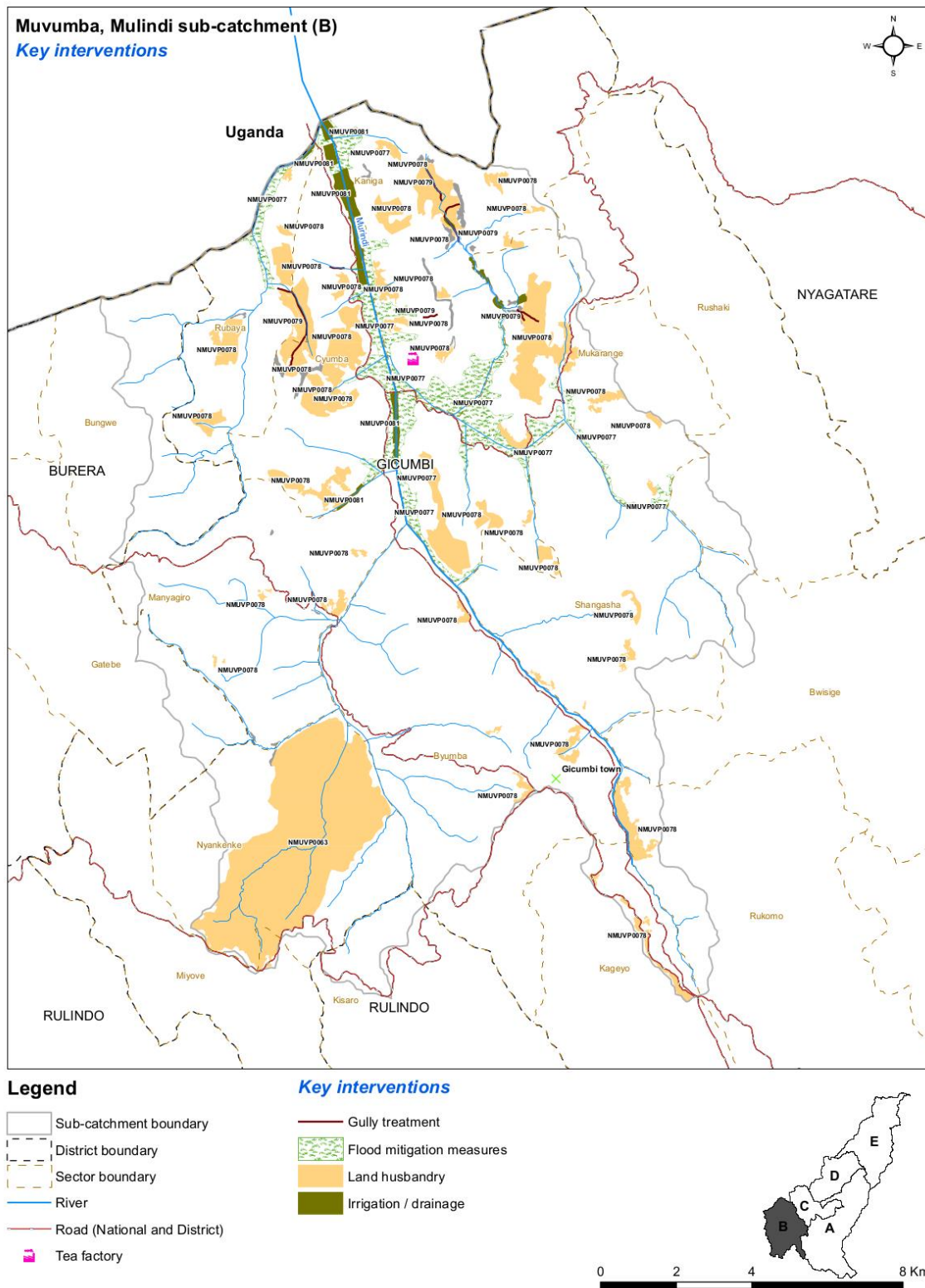
Figure 51: Key interventions in Mulindi sub-catchment (interventions included only where spatial scope is known)
