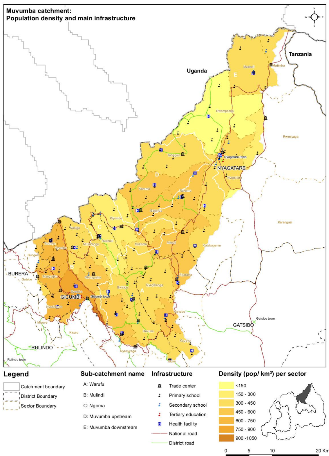
Figure 42: Muvumba catchment population density and key-infrastructure
