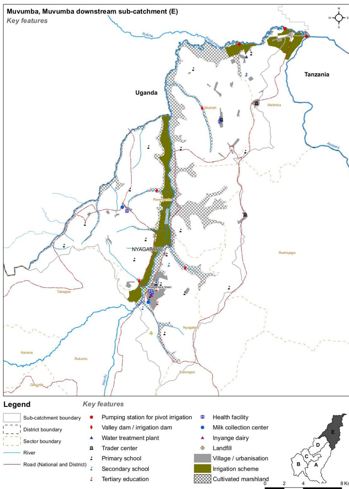
Figure 48: Key geographic features of the Muvumba Downstream Catchment
